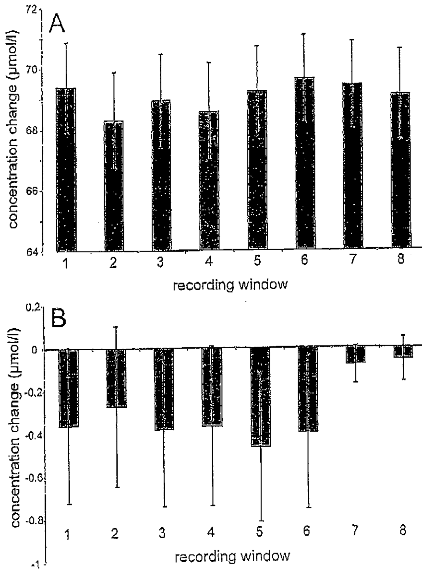
Fig. 3. Concentration changes of TOI (panel A) and of CYT-c (panel B) in the eight observation windows. The TOI decreases during blood drawing (2 nd window) and then raises back to the baseline levels. The CYT-c markedly increases in the 7 th window (1 hour from the end of the blood reinjection).
